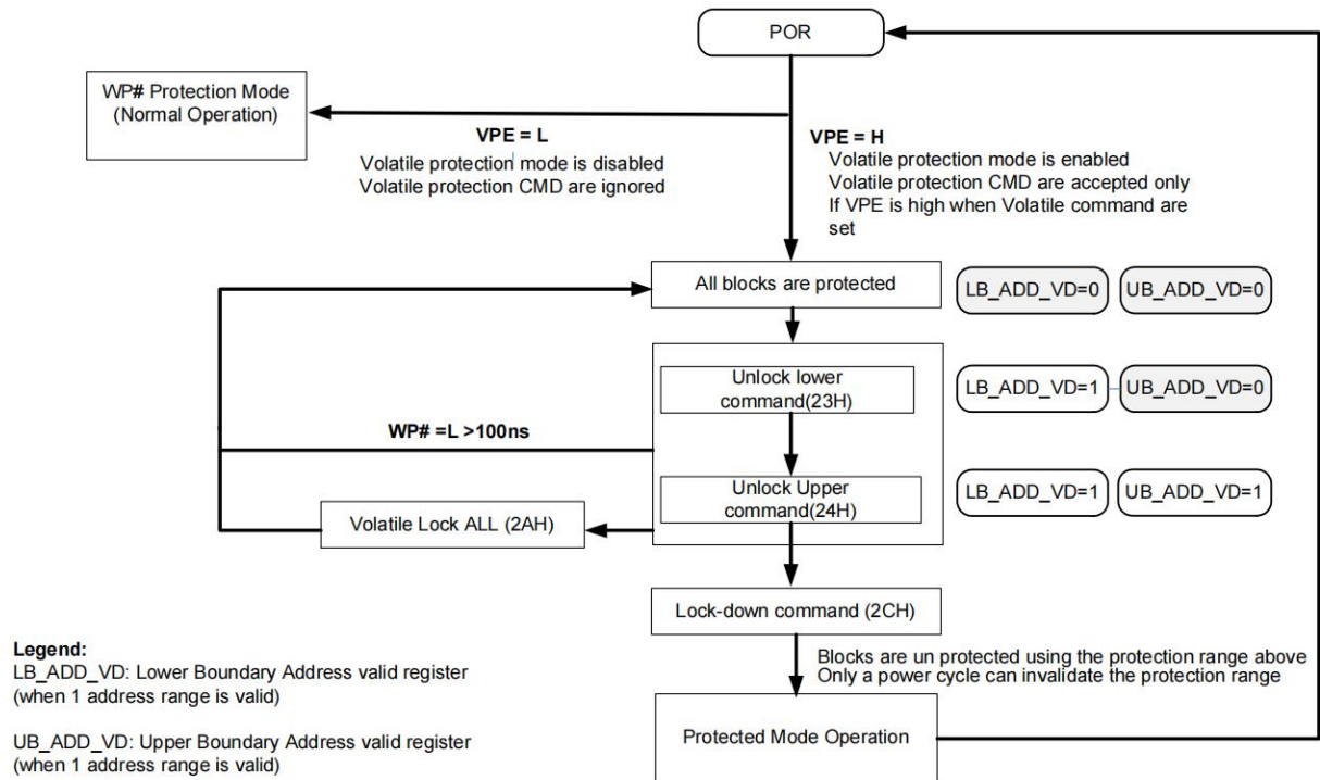
Figure 5. VBP Flowchart
