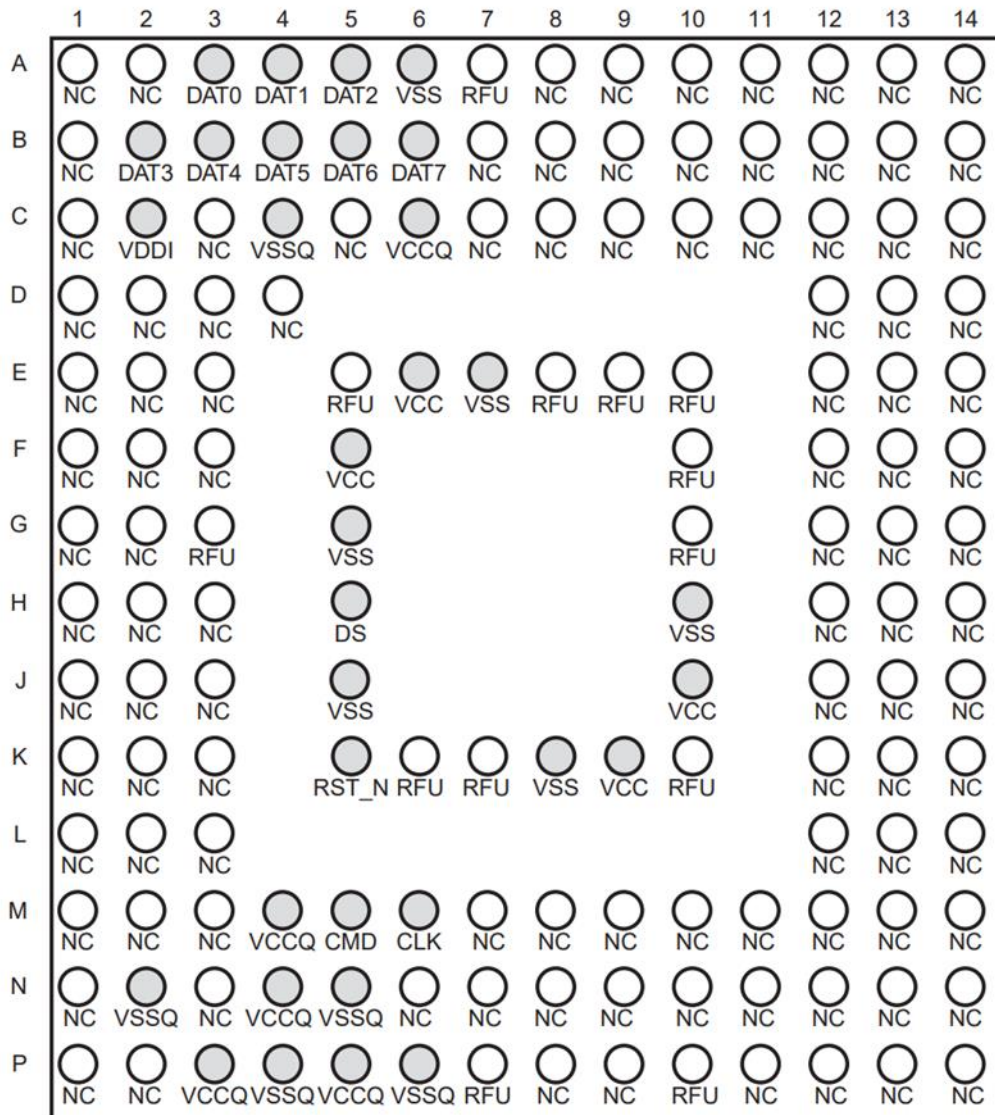
FBGA153 Package Connection (top view through package)
